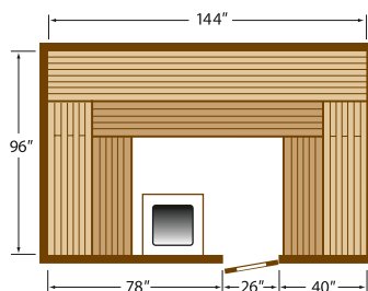
FPC 812 Your Interior Framing Dimensions Seats 12 people. K15G Heater.
